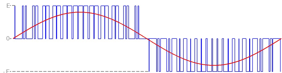
FIGURE 4 Line-to-line voltage in a conventional 2-level inverter
